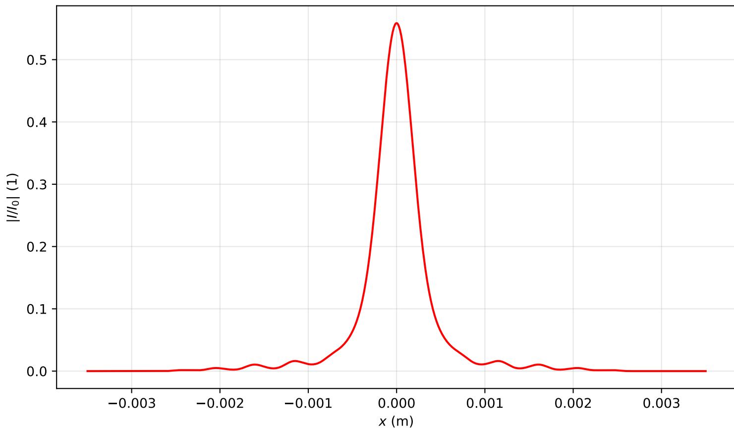
Intensity profile I(x, y = 0, z = 3.025)/I_0 , \text{Pin}=3.0\text{Pcr} , artificial time
